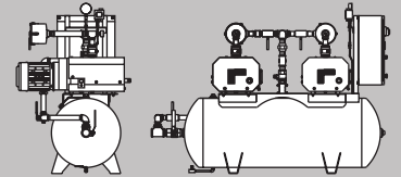
Horizontal Tank Mounted Duplex
